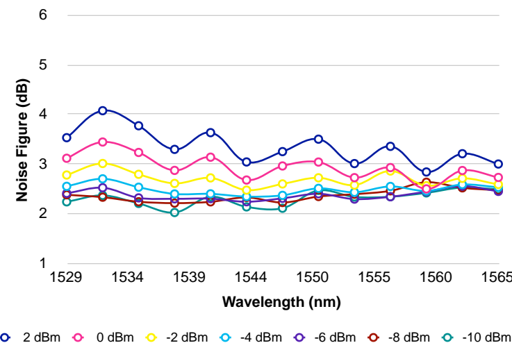
AEDFA-C-PM-30-B-FA Noise Figure
