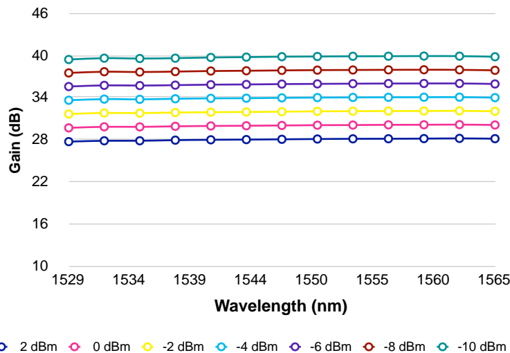
AEDFA-C-PM-30-B-FA Gain
